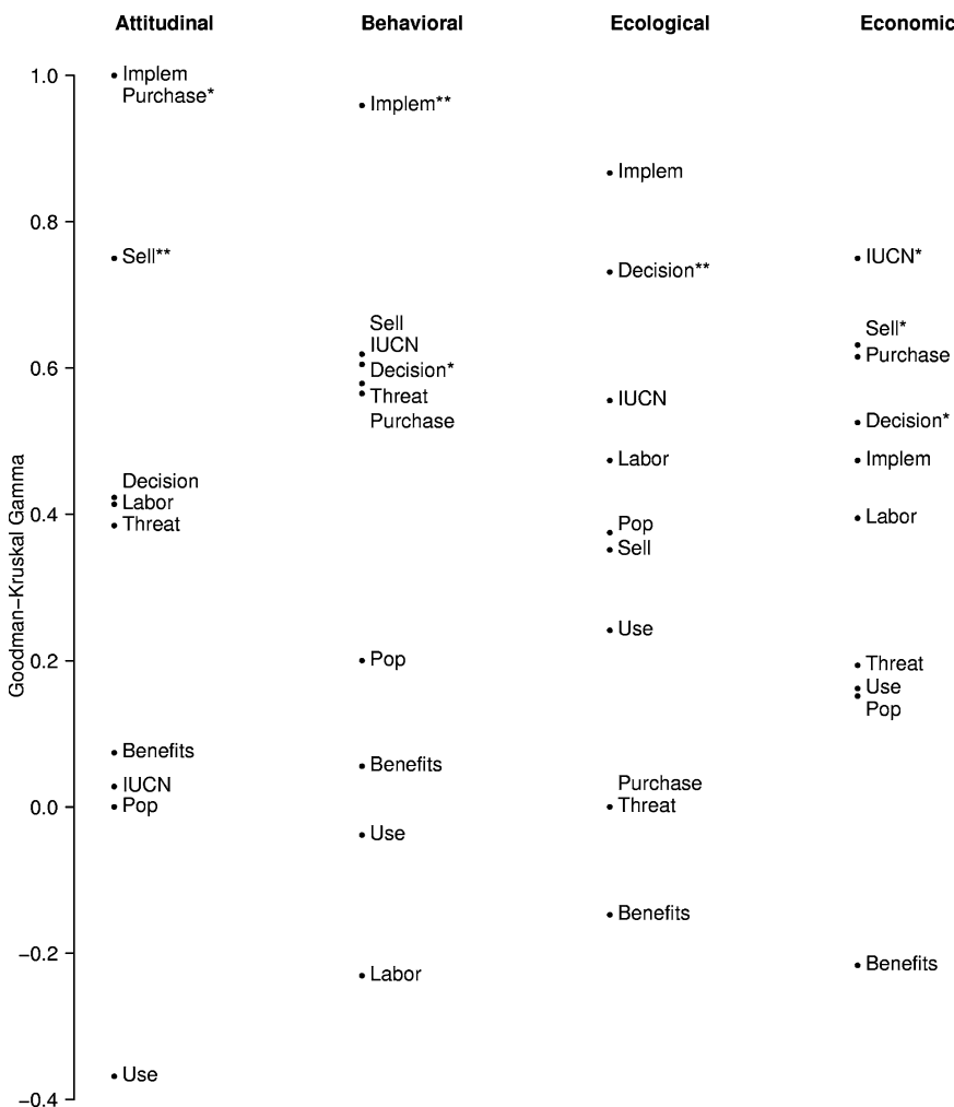
Figure 1. Goodman–Kruskal gamma statistics for contingency tables of predictors (in columns) and outcomes (column headings). The value of gamma for the table is plotted along the y-axis. Gamma relatively close to 1 indicates a positive association between the ordinal levels of predictor and outcome. Double asterisks indicate tables with q values in (0, 0.05), single asterisks q values in (0.05, 0.1). The eight tests having one or two asterisks are called significant. Significance levels are adjusted for the false discovery rate of the series of tests as described in the text (Implement denotes the variable implementation, and Pop denotes population).
